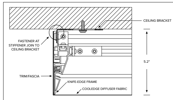
SURFACE MOUNT
