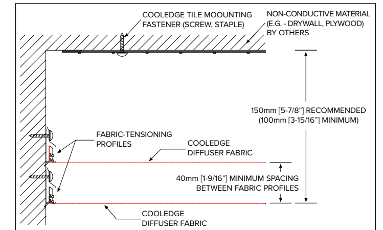
FLUSH MOUNT
