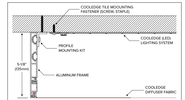
SURFACE MOUNT - CURVED/ROUND/CIRCLE
