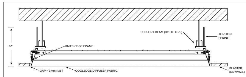
RECESSED
