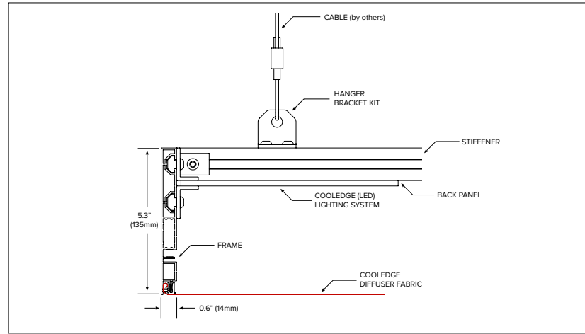
SUSPENDED (ROUNDS)
