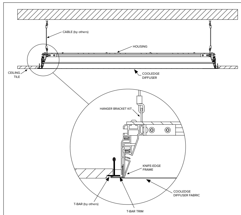
GRID (T-BAR)
