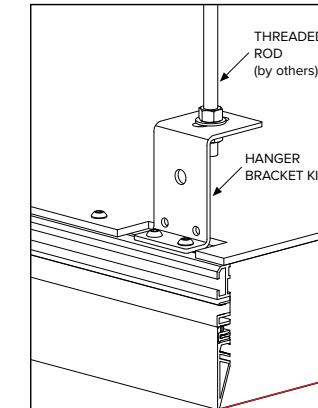
SUSPENDED (THREADED ROD OPTION)
